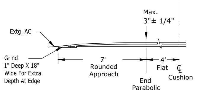
SECTION VIEW A - A Symmetrical About \zeta N.T.S.
