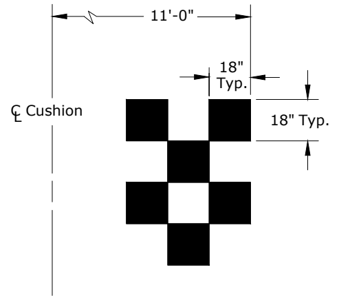
PAVEMENT MARKING DETAIL N.T.S.
