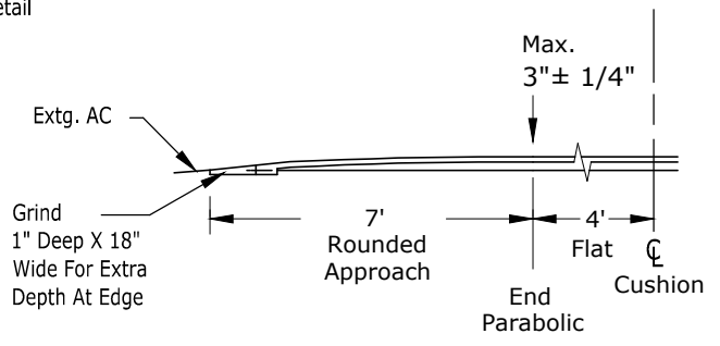
SECTION VIEW A - A Symetrical About \zeta N.T.S.
