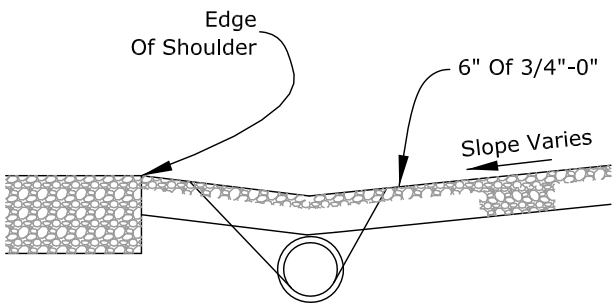
TYPICAL SECTION GRAVEL DRIVEWAY AT GRAVEL ROAD
