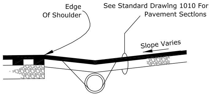
TYPICAL SECTION A.C. DRIVEWAY AT A.C. ROAD
