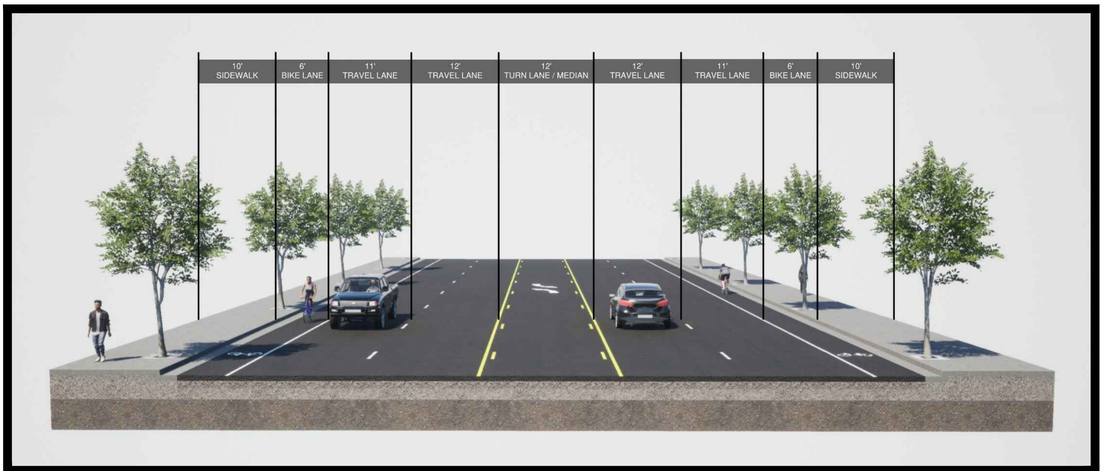
WALKER ROAD - 5 LANE SECTION (STANDARD TYPICAL SECTION - CITY OF BEAVERTON)
