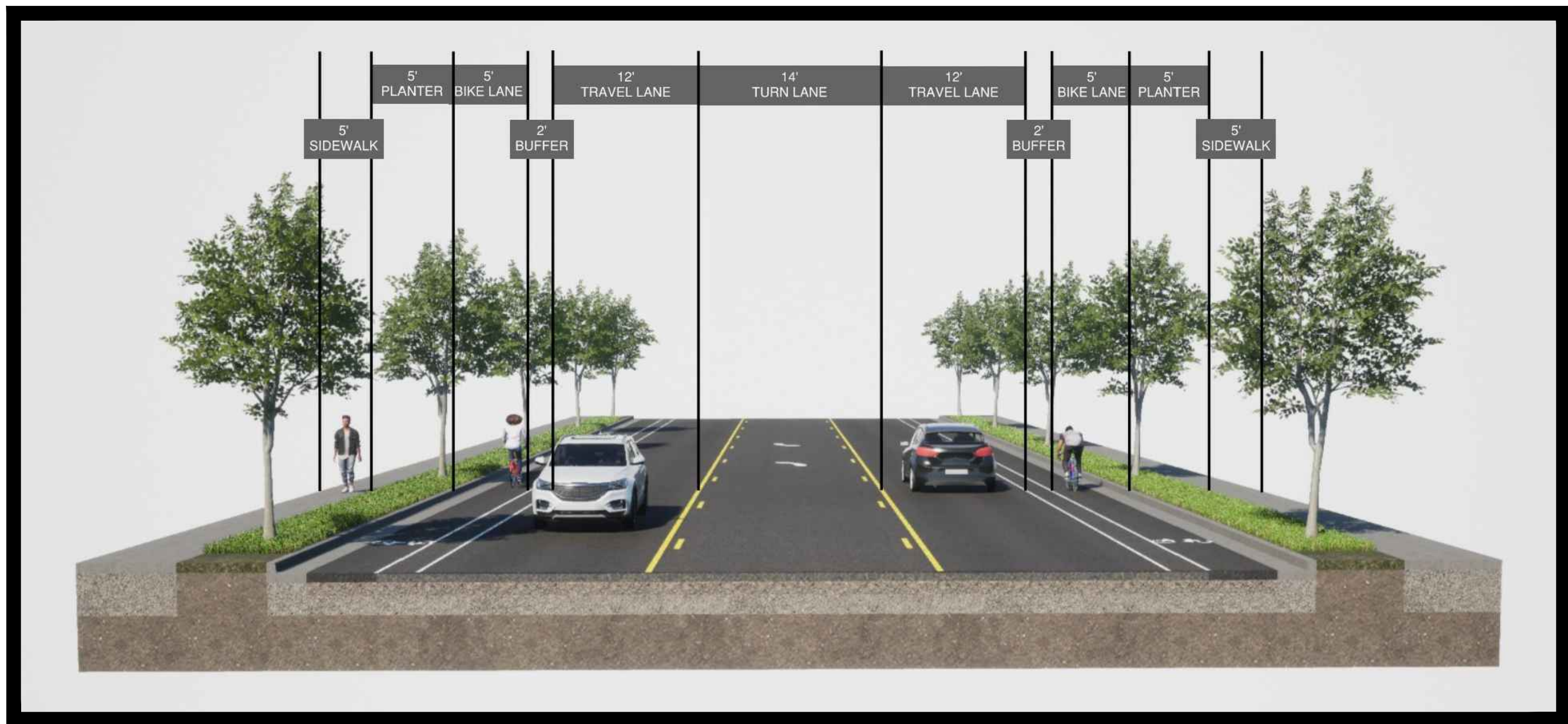
WALKER ROAD - 3 LANE SECTION (STANDARD TYPICAL SECTION - WASHINGTON COUNTY)
